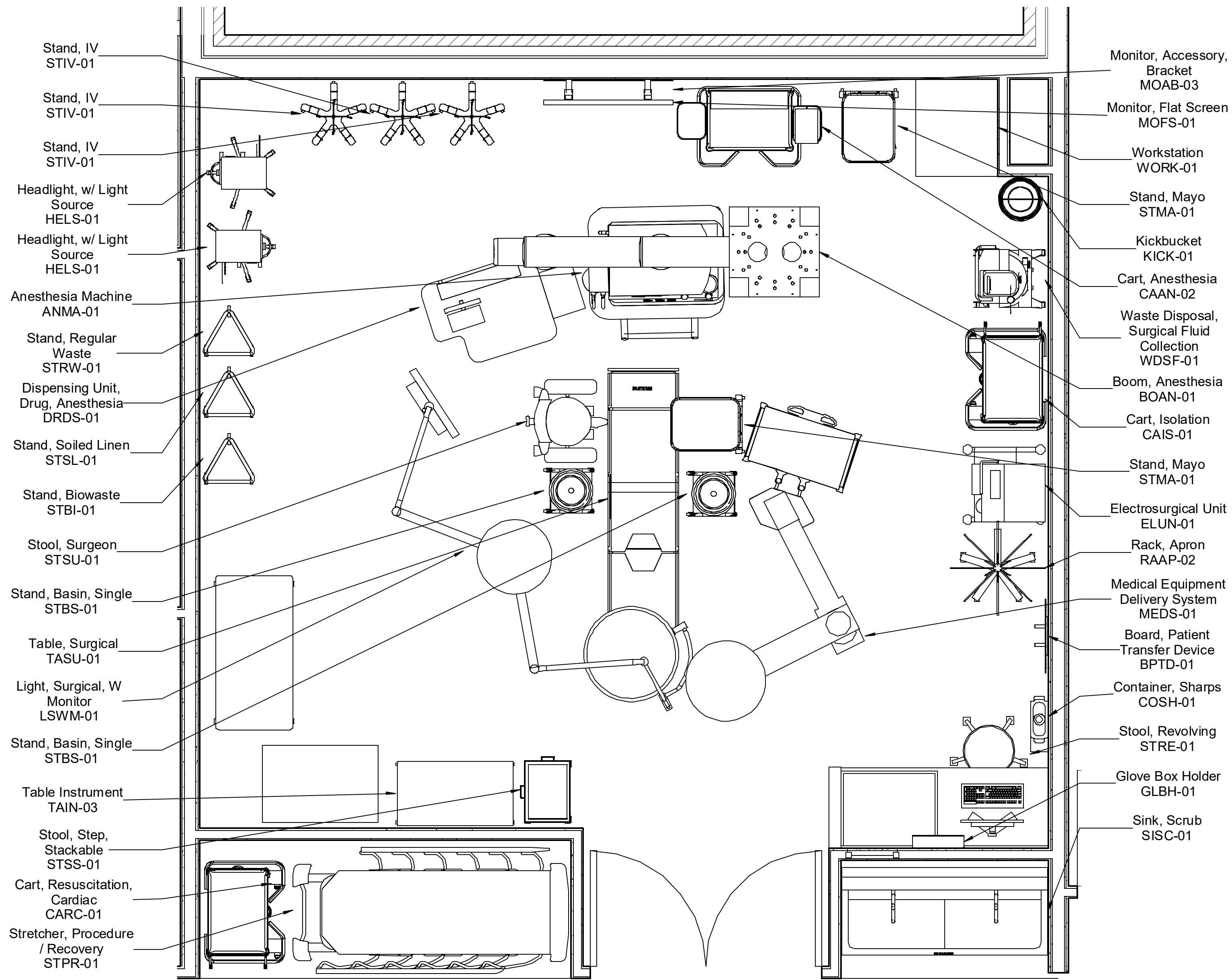
2 SR- OR 1/2" = 1'-0"
